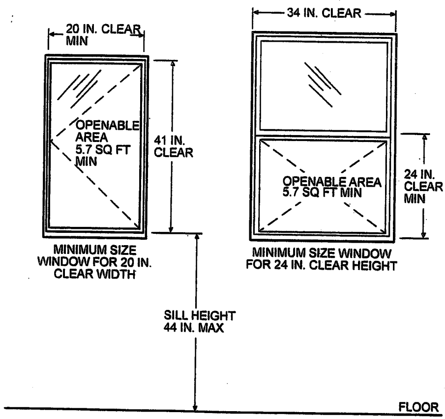
Figure R310.1 EMERGENCY ESCAPE AND RESCUE WINDOW
