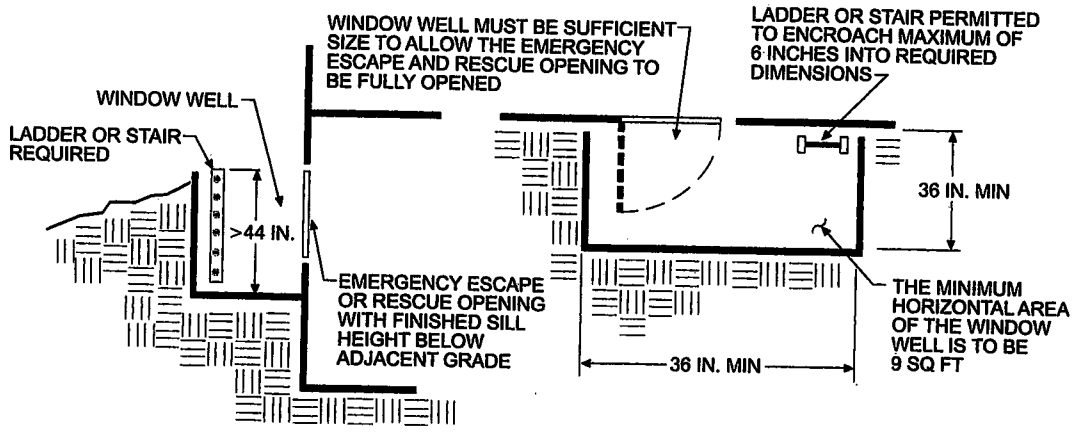
Figure R310.2 WINDOW WELLS
